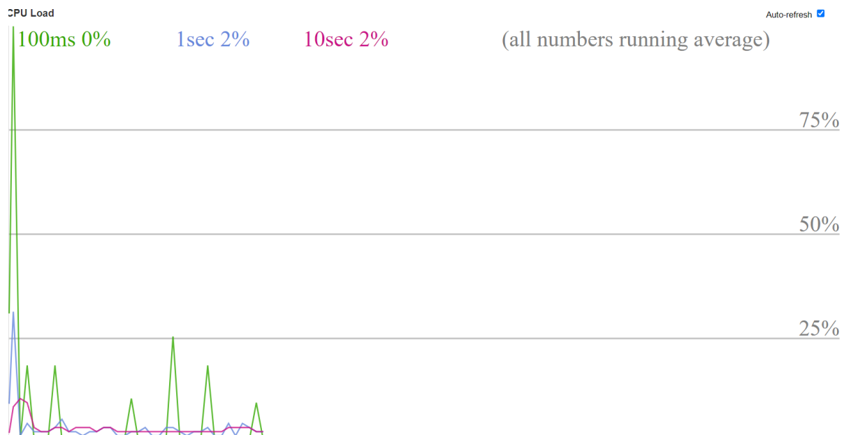
Figure 3-1.3: CPU Information
