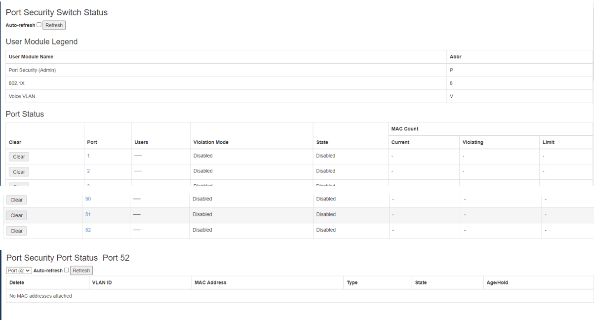
Figure 3-9.2.1.1: The Port Security Switch Status
